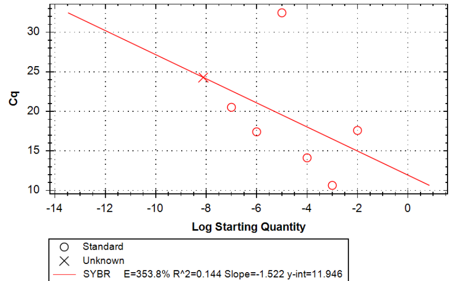
Standard Curve
