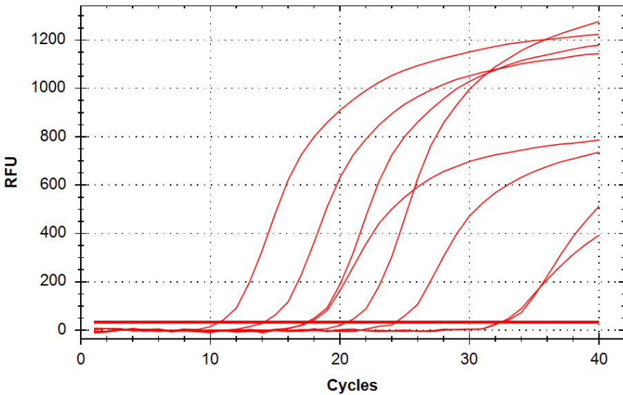
Amplification
