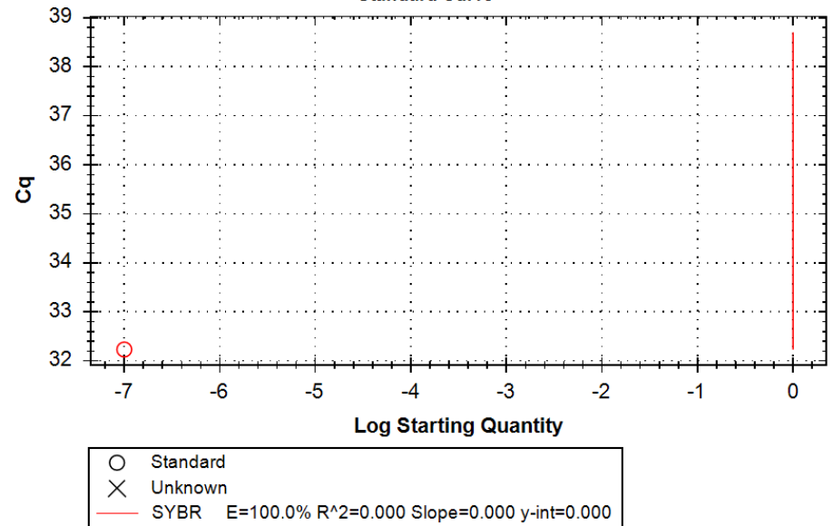
Standard Curve
