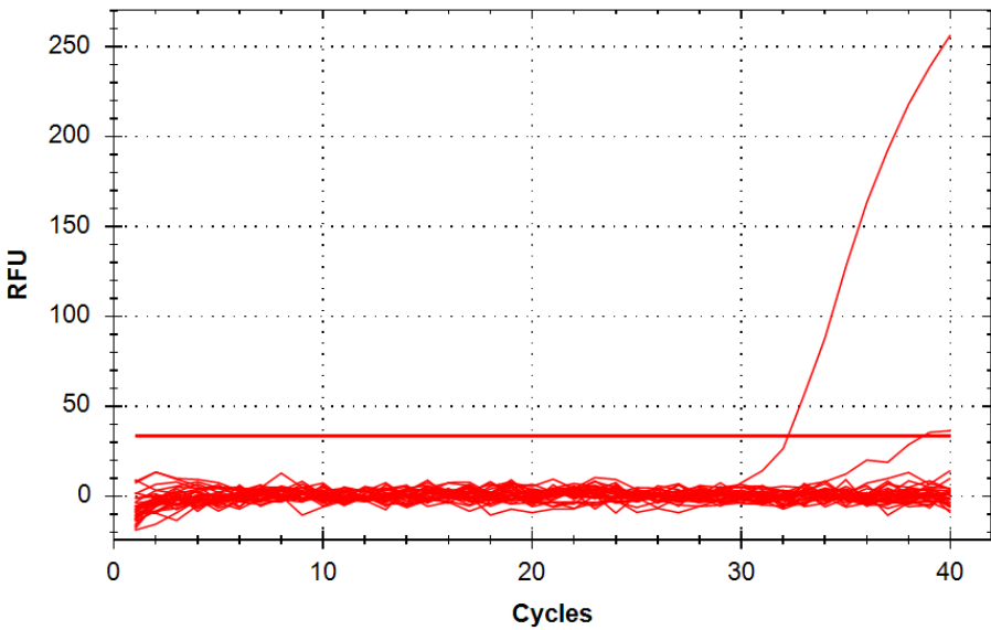
Amplification
